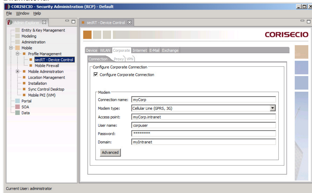
Screenshot – Administration of the securityRunTime
